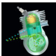
STIHL 2-MIX-Motor
